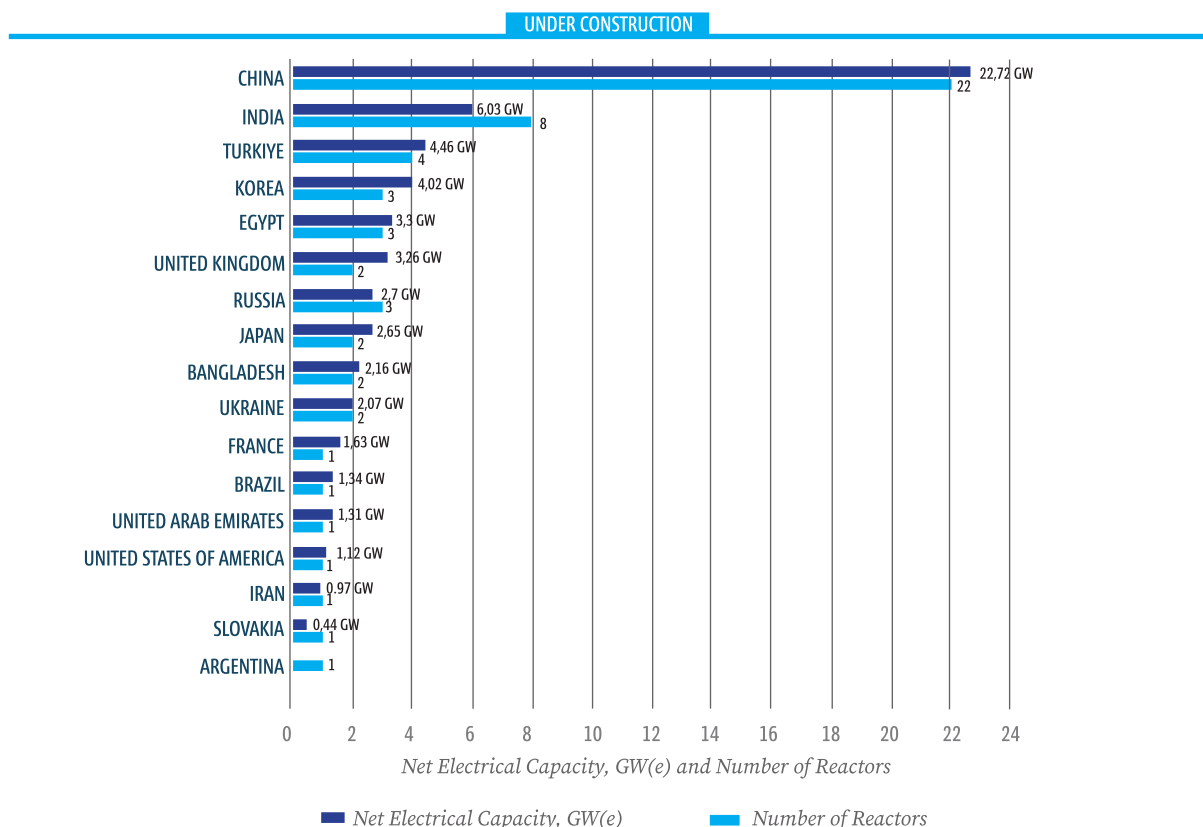
Number of nuclear reactors under construction by country
